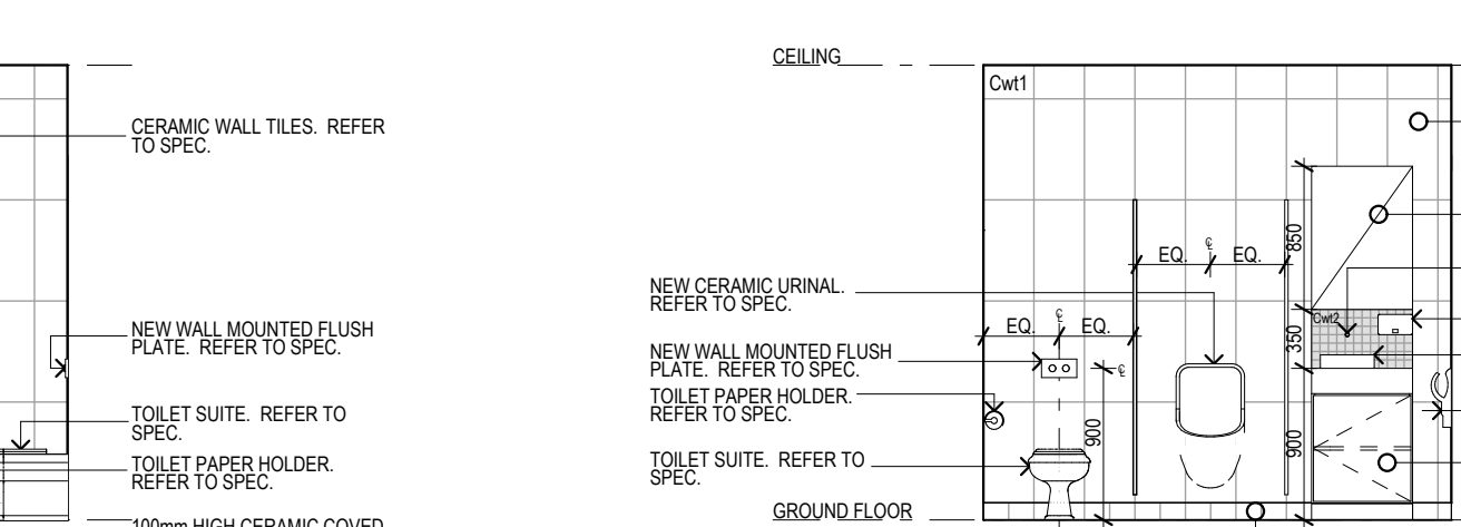
2.008 MALE WC SCALE 1:50 0mm 500 1000 1500 2000 2500
