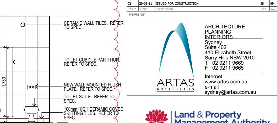
2.005 FEMALE WC SCALE 1:50 0mm 500 1000 1500 2000 2500
