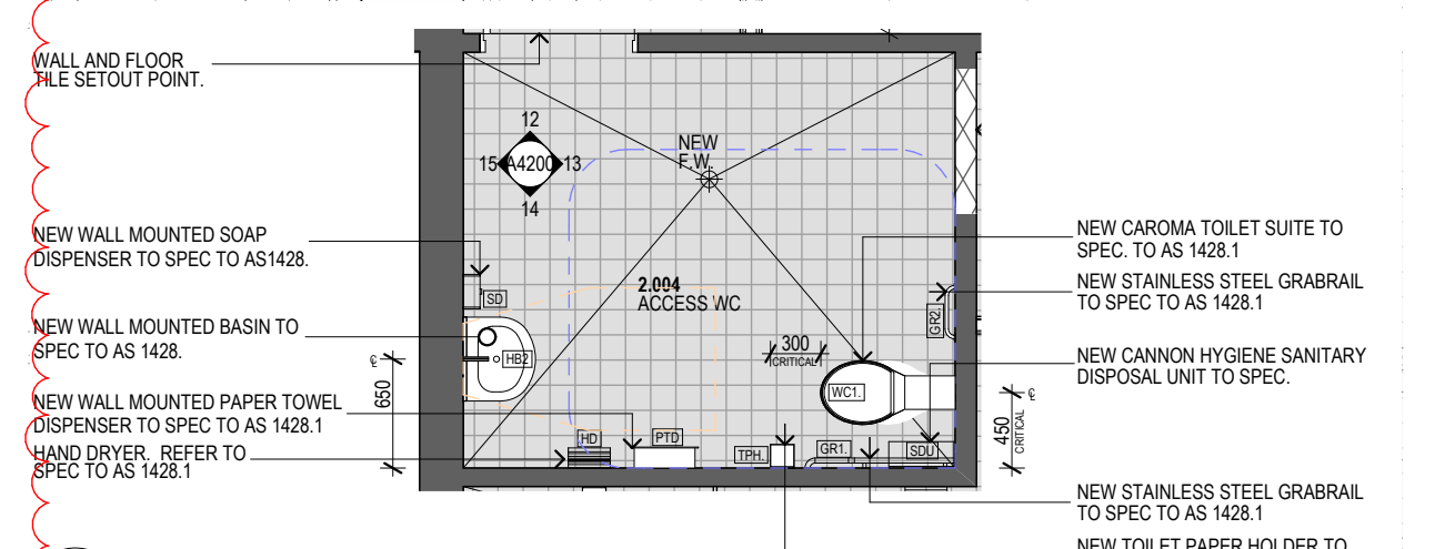
2.004 ACCESS WC SCALE 1:50 0mm 500 1000 1500 2000 2500
