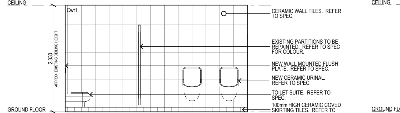
1.007 EX. MALE WC SCALE 1:50 0mm 500 1000 1500 2000 2500
