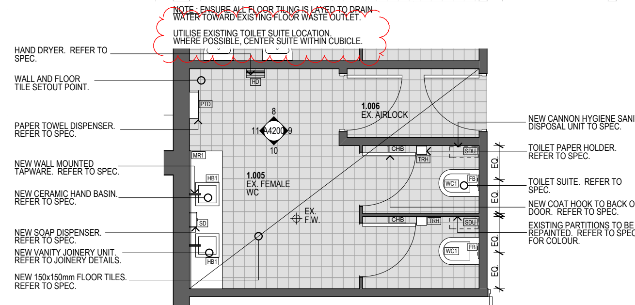
1.005 EX. FEMALE WC SCALE 1:50 0mm 500 1000 1500 2000 2500
