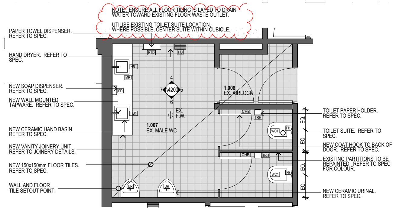
1.007 EX. MALE WC SCALE 1:50 0mm 500 1000 1500 2000 2500
