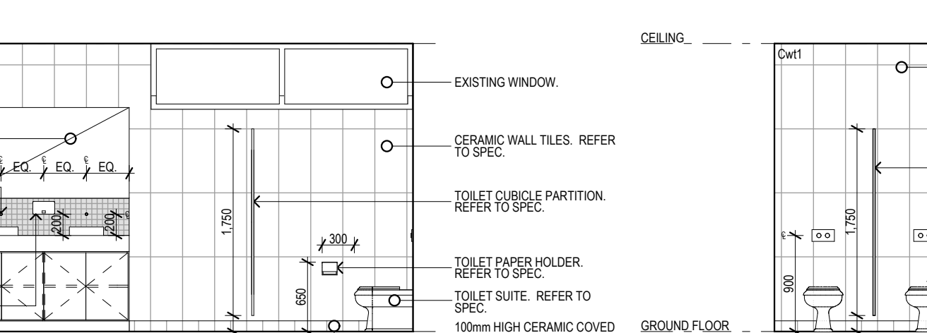
2.005 FEMALE WC SCALE 1:50 0mm 500 1000 1500 2000 2500
