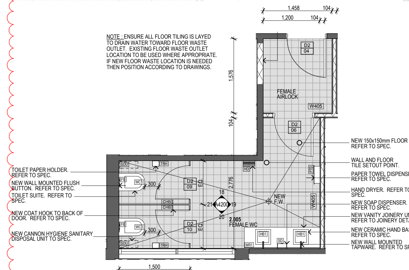
2.005 FEMALE WC & AIRLOCK SCALE 1:50 0mm 500 1000 1500 2000 2500
