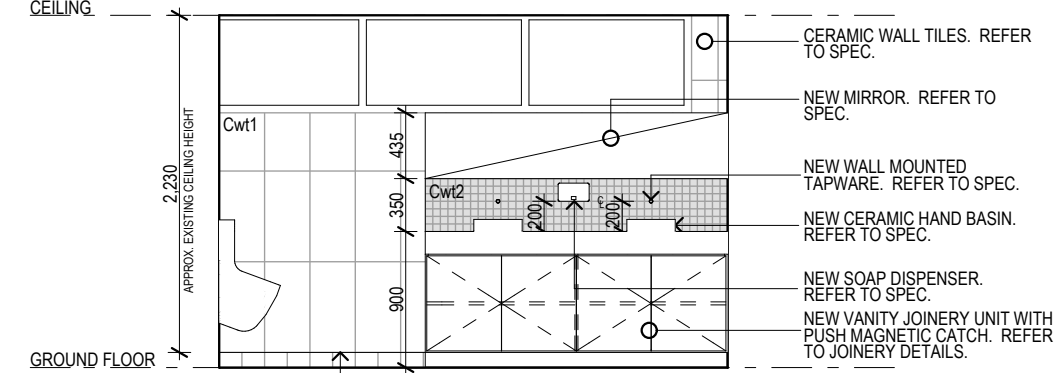
1.007 EX. MALE WC SCALE 1:50 0mm 500 1000 1500 2000 2500
