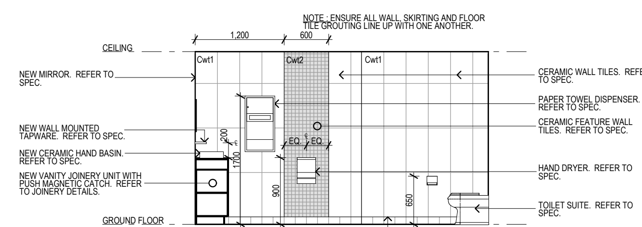
1.007 EX. MALE WC SCALE 1:50 0mm 500 1000 1500 2000 2500
