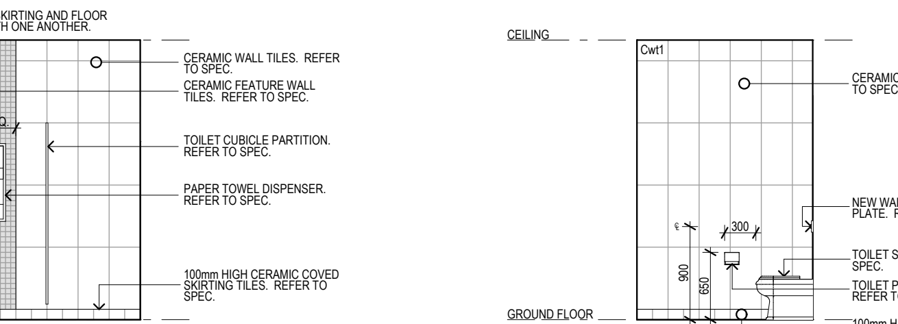
2.008 MALE WC SCALE 1:50 0mm 500 1000 1500 2000 2500
