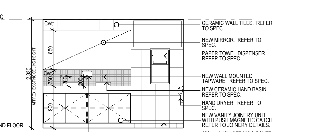
1.005 EX. FEMALE WC SCALE 1:50 0mm 500 1000 1500 2000 2500
