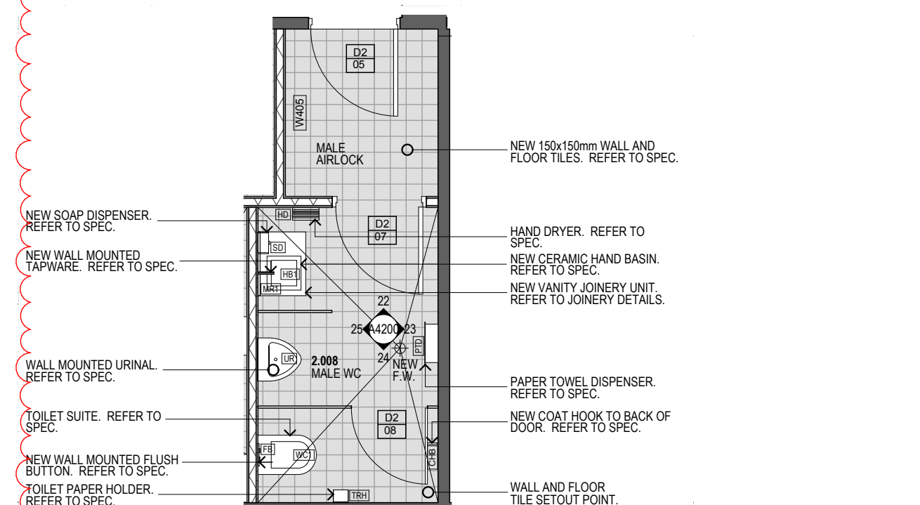
2.008 MALE WC & AIRLOCK SCALE 1:50
