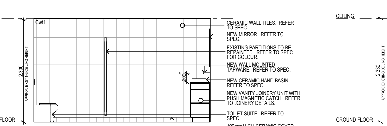
1.005 EX. FEMALE WC SCALE 1:50 0mm 500 1000 1500 2000 2500
